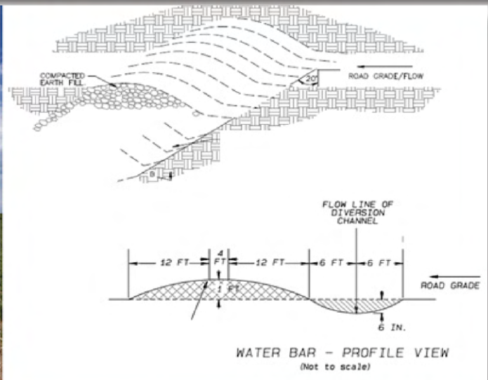
A water bar built in the low point of the road can stabilize drainage and keep fine sediment out of the gully bottoms
